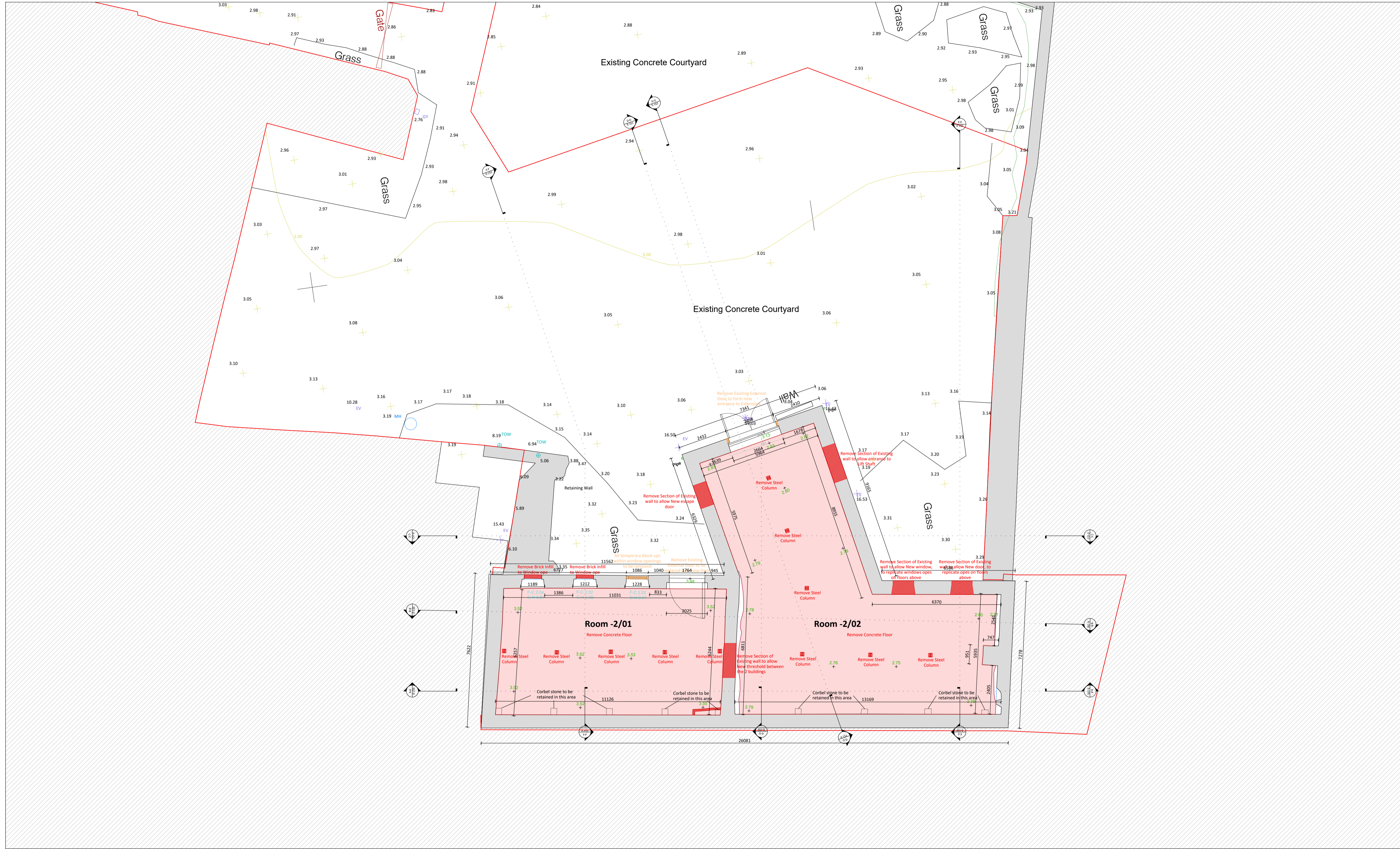
01 Level -2 (Plaza) Demolition Floor Plan As Existing Scale: 1:100
